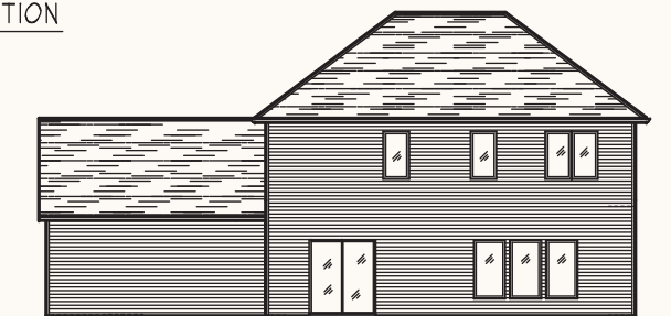
REAR ELEVATION
